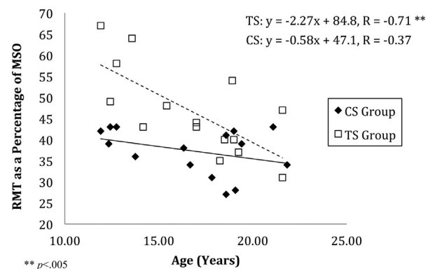
Fig. 2. Resting motor threshold (RMT) calculated as percentage of maximum stimulator output (MSO) to elicit a motor evoked potential (MEP) of between 150 and 200 \mu\text{V} plotted against the age of participant. A stepwise regression was conducted and showed that both group and age was predictive of RMT ( F(2, 31) = 17.03, p < .0001 ). These two factors explained roughly 50% of the variance ( R^2 = 0.524 , Adjusted R^2 = 0.493 ).
